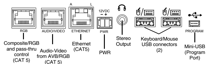
FIG. 2 Connector layout on the 1500VG Touch Panels
